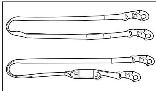
Figure 4: SM/RTC 8250-P6HH & SM/RTC 8252-P6HH
