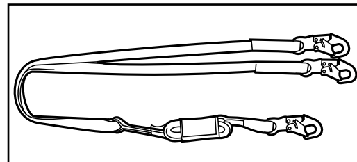
Figure 5: SM/RTC 8252 Series “Y” Lanyard for continuous protection
